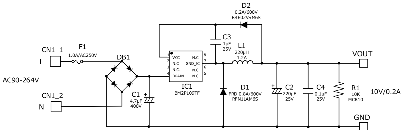
Figure 3. BM2P109TF-EVK-001 Schematics
