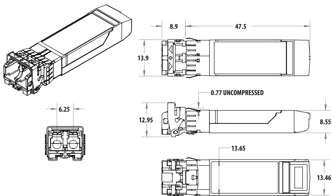
Figure 5. Module drawing.
