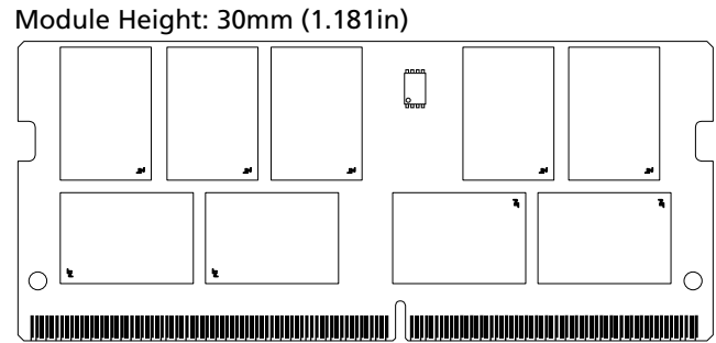
Figure 1: 260-Pin SODIMM (MO-310 R/C H)
