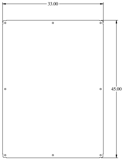
INNER PANEL
