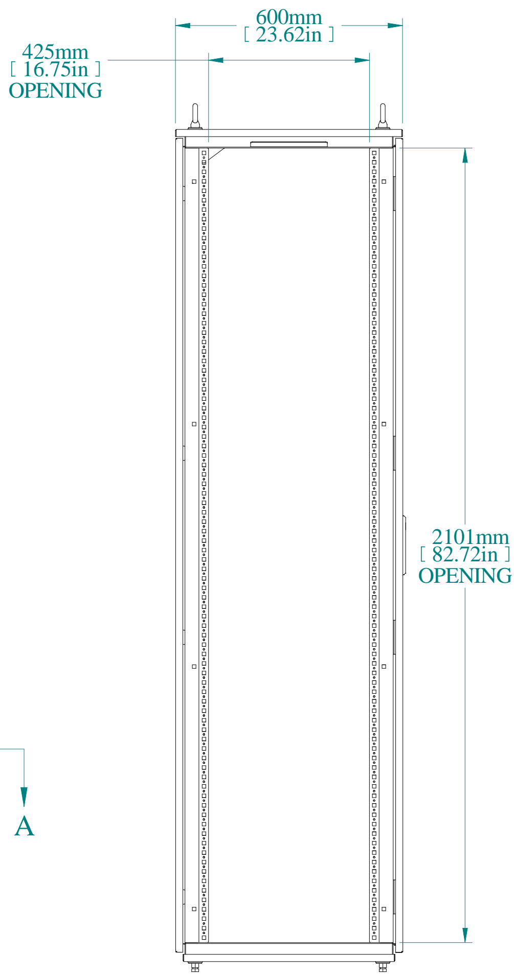
L.S. VIEW
