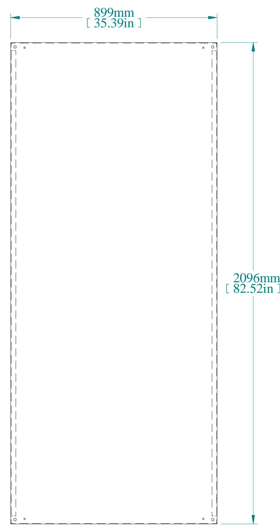
INNER PANEL
