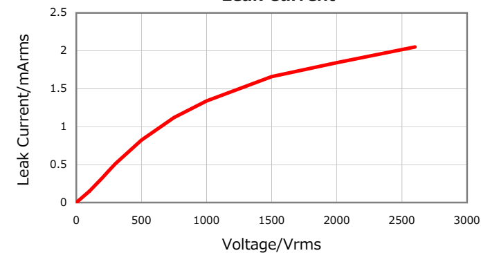
Leak Current
