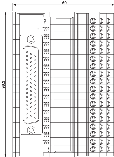
Dimensional drawing
